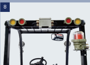
Explosion proof type LED rear work lamp
